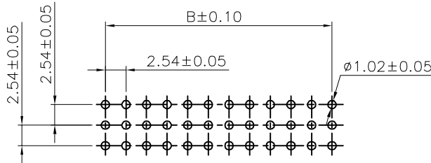
PCB LAYOUT(RECOMMENDED) (TOP VIEW TOL. :±0.05)
